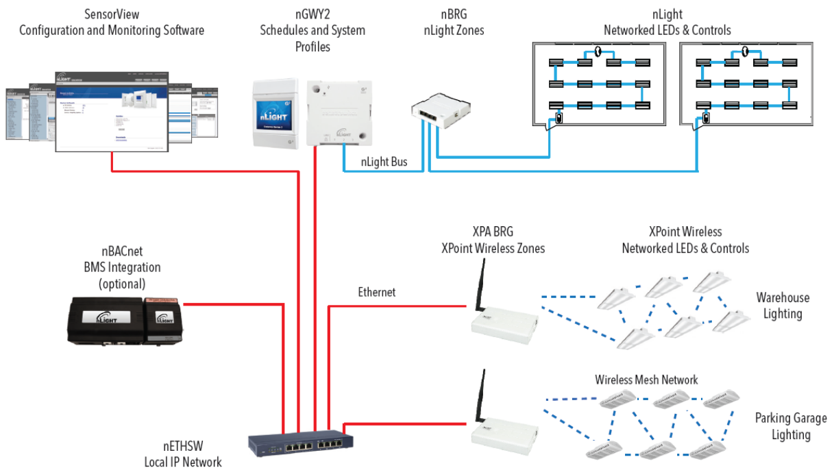
Figure 1 - Example Typical nLight System Riser Diagram
