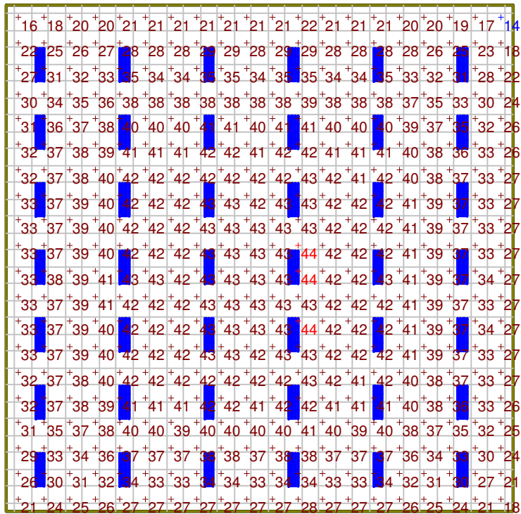
TYPICAL 60' X 60' X 12' AREA
